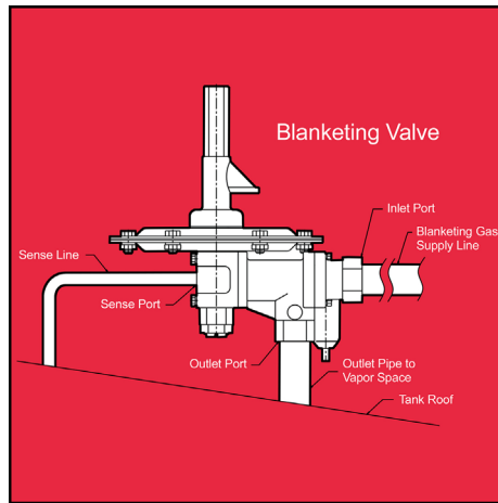
A tank blanketing valve controls the flow rate of nitrogen based on pressure. Source: Protectoseal
