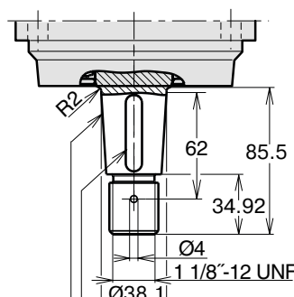
Key 9.54x9.54x44.45 Tapered key shaft "V" SAE J744 38-3 (C-C)
