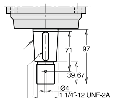
Key 11.11x11.11x50.8 Tapered key shaft "V" SAE J744 44-3 (D&E)
