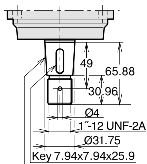
Key 7.94x7.94x25.9 Tapered key shaft "V" SAE J744 32-3 (C)
