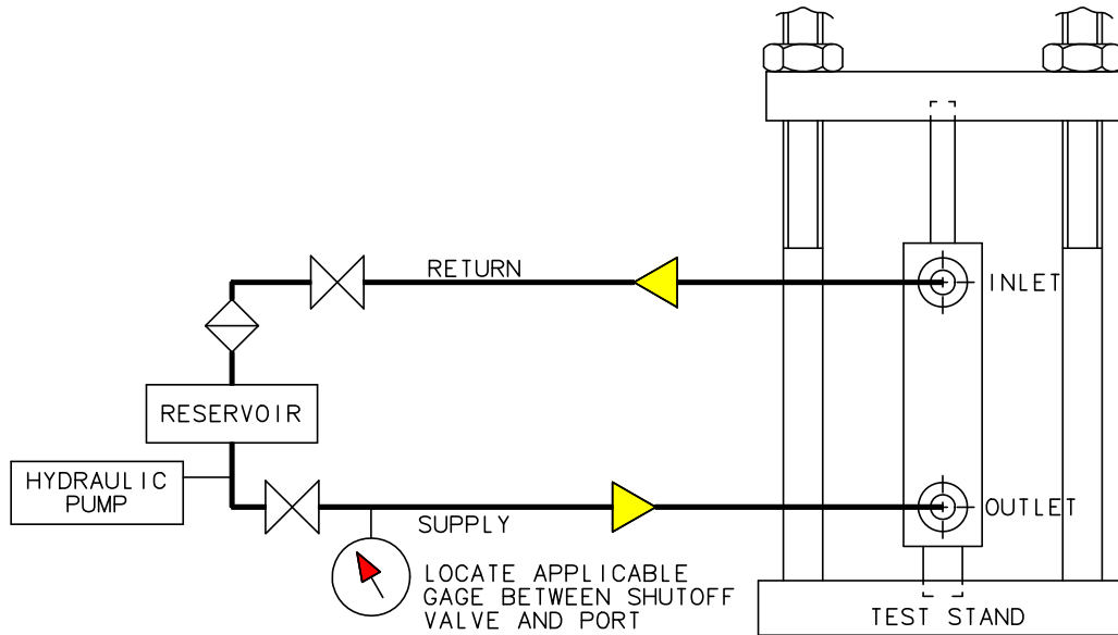
Test Setup - Figure 2
