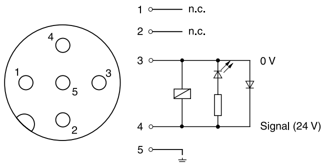
M12 pin assignment, code „DL“, surge diode with LED 1) , pins 1 and 2 not connected
