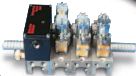
ISU on Valvair II manifold
